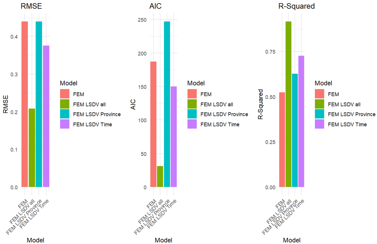
Figure 3. Model Accuracy
