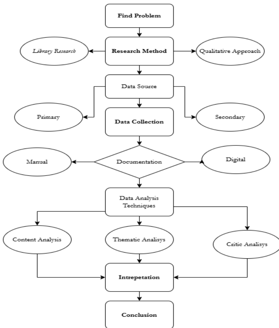
Figure 1. Research Flow
