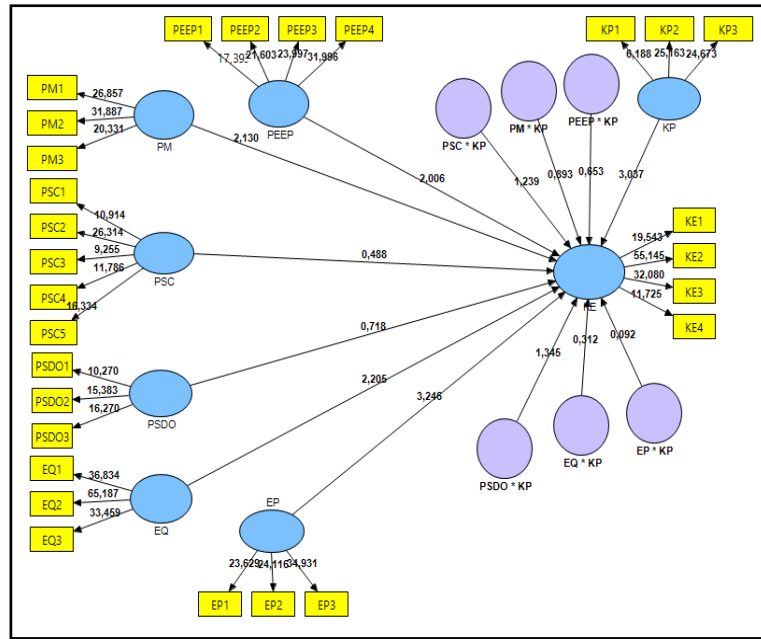
Figure 3. Bootstrapping Result
